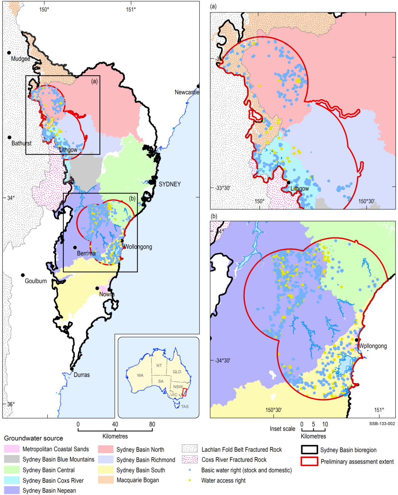
Figure 22 Location of groundwater elements within the preliminary assessment extent (PAE) of the Sydney Basin bioregion
