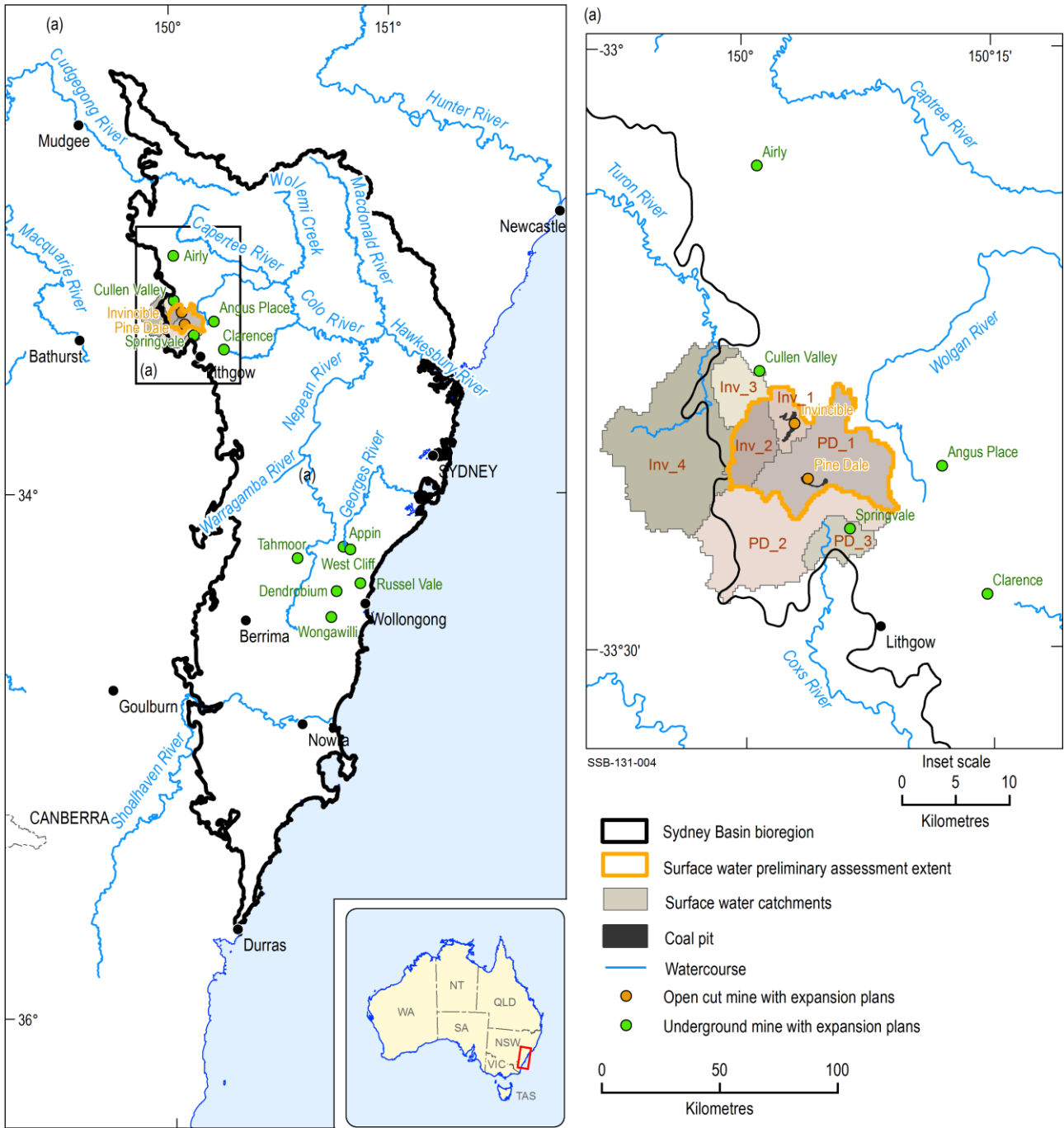
Figure 6 Features used to calculate the surface water preliminary assessment extent (PAE) in the Sydney Basin bioregion
