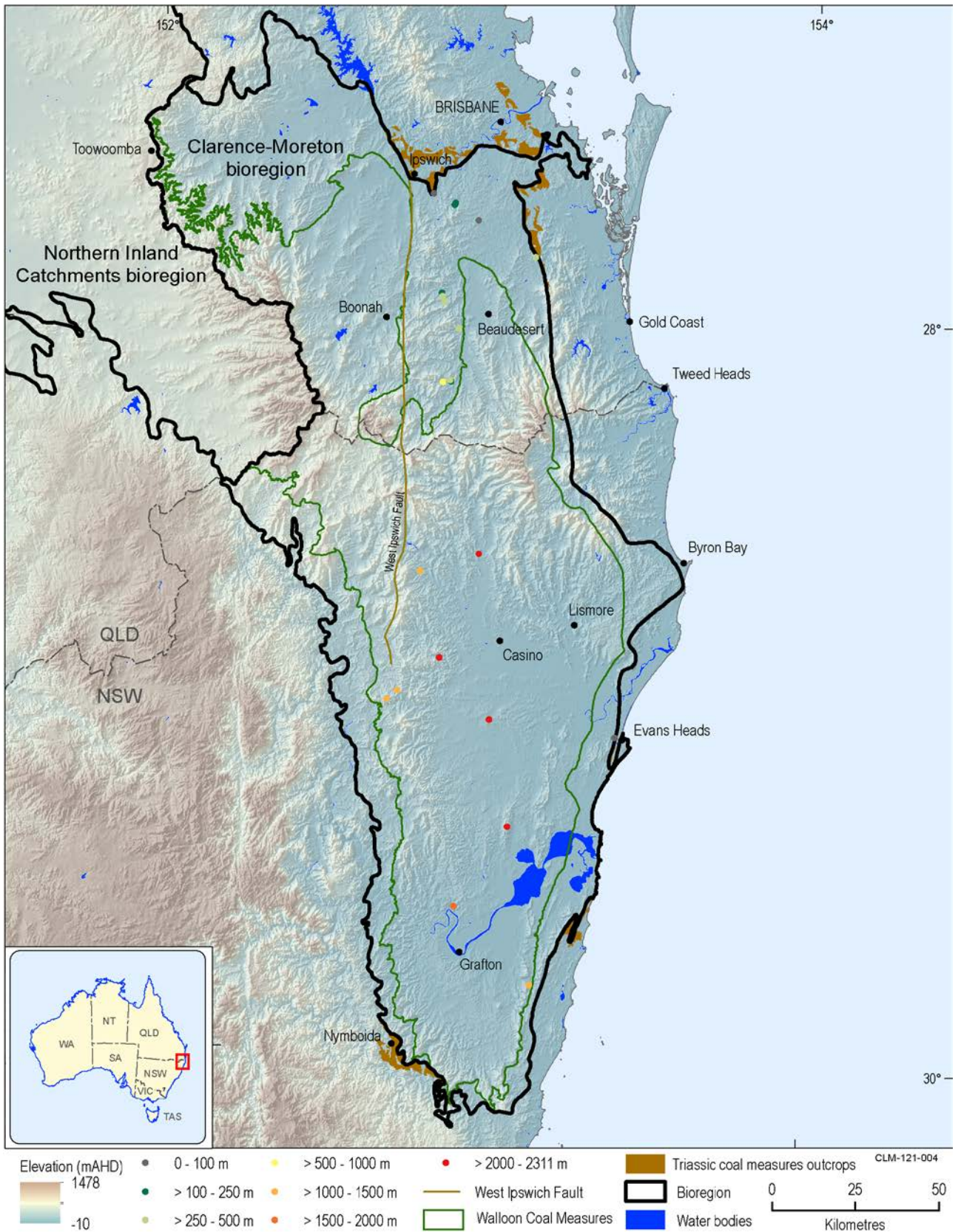
Figure 6 Depth to the top of the Ipswich Coal Measures (and equivalents) intersected at exploration and stratigraphic wells in the Clarence-Moreton bioregion. The Ipswich Coal Measures are absent west of the West Ipswich Fault. The extent of the Walloon Coal Measures is shown for comparison
