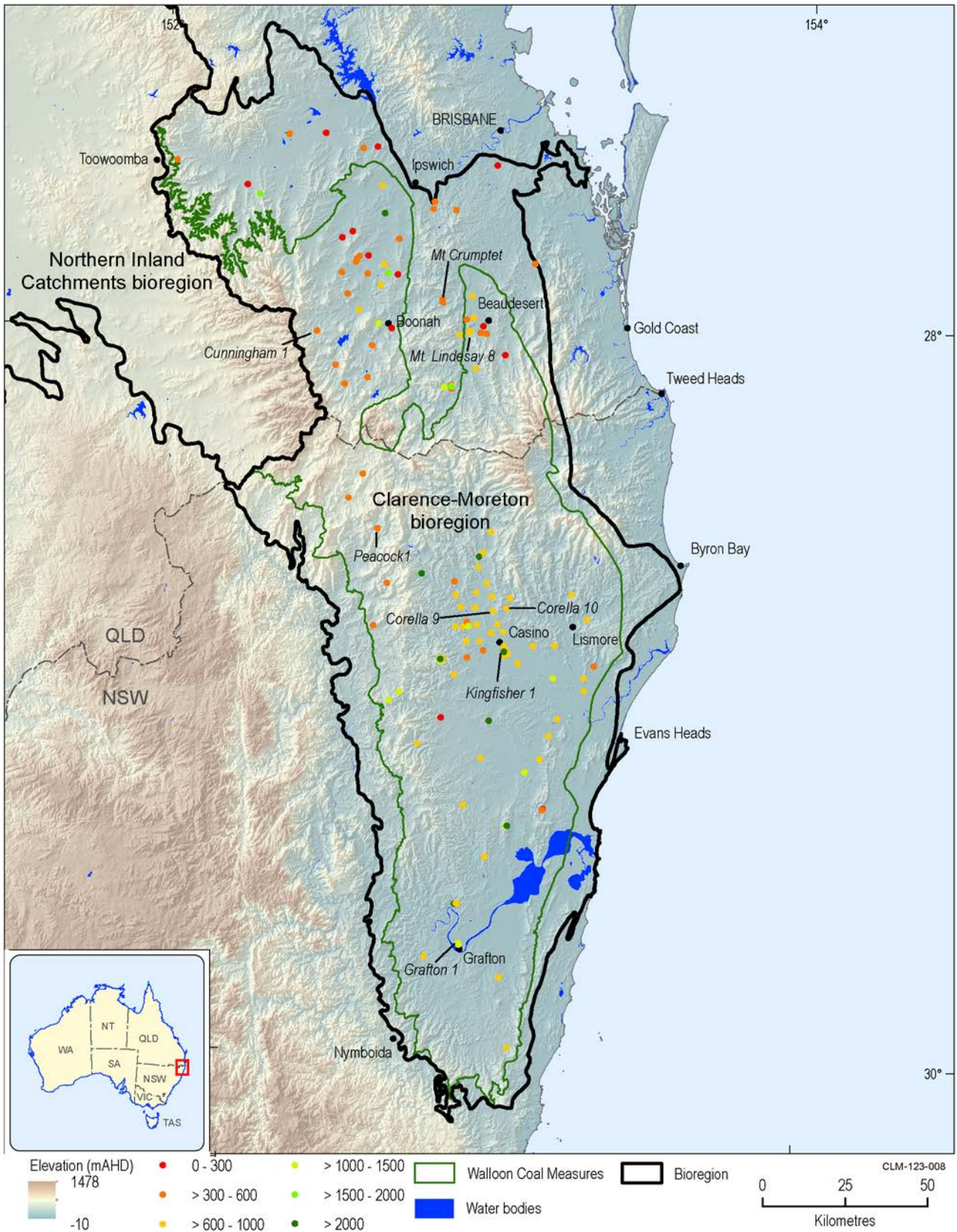
Figure 9 Spatial distribution and depth of coal seam gas and petroleum exploration wells in the Clarence-Moreton bioregion. Wells drilled outside the boundary of the Walloon Coal Measures target the older coal seams (i.e. Ipswich Coal Measures).
