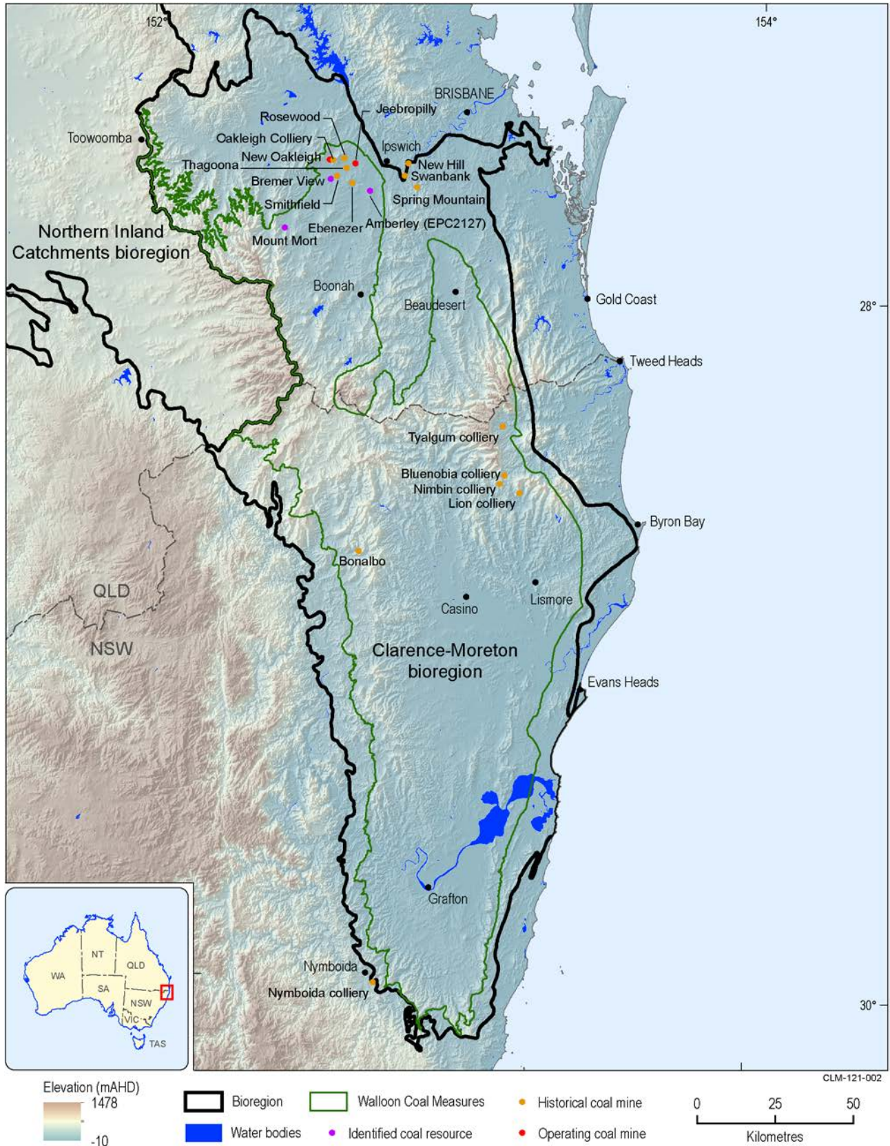
Figure 4 Identified coal resources and operating and historical coal mines in the Clarence-Moreton bioregion (additional historical coal mines in Queensland that are not included in the OZMIN database are described in Cameron, 1970)
