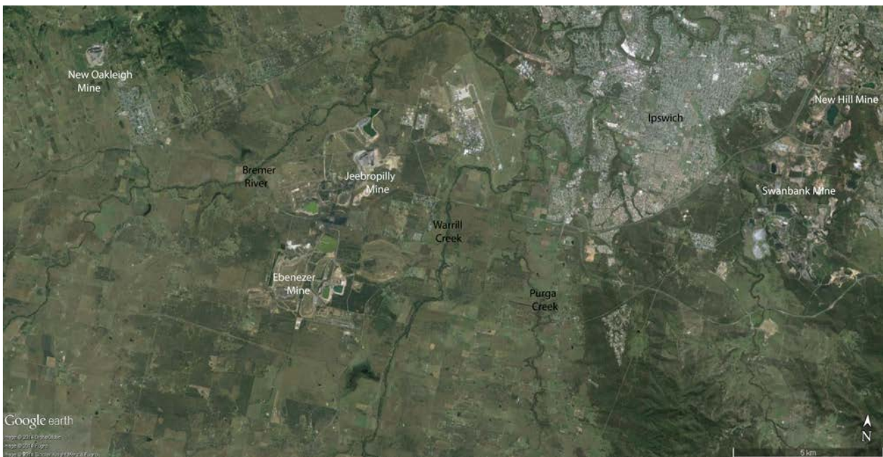
Figure 8 Active and historical coal mines in south-east Queensland in the Clarence-Moreton bioregion
