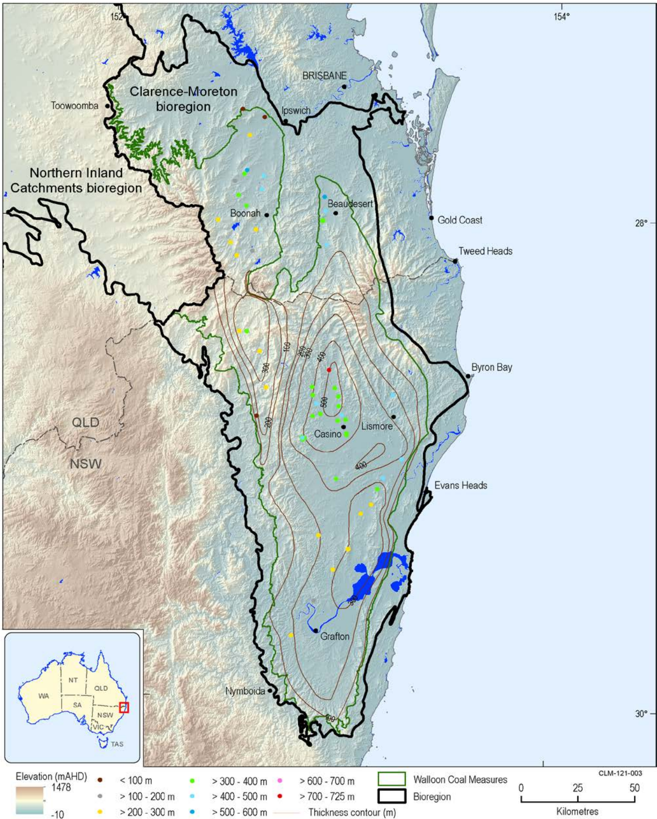
Figure 5 Isopach (thickness) map of Walloon Coal Measures (Ingram and Robinson, 1996) and comparison with thickness of Walloon Coal Measures recorded at coal seam gas, coal exploration, petroleum exploration and stratigraphic wells in the Clarence-Moreton bioregion
