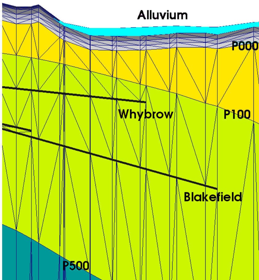
Figure 9 Cross-section through part of Bulga coal mining area, including the alluvium (light blue) and Whybrow and Blakefield coal seam discs (bold black lines)
