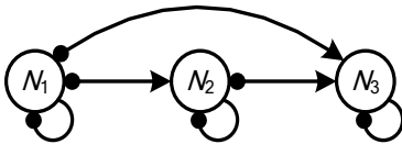
Figure 5 A signed digraph of a predator–prey community of size n = 3 , where the top predator N_3 is an omnivore that feeds on the two other prey species
