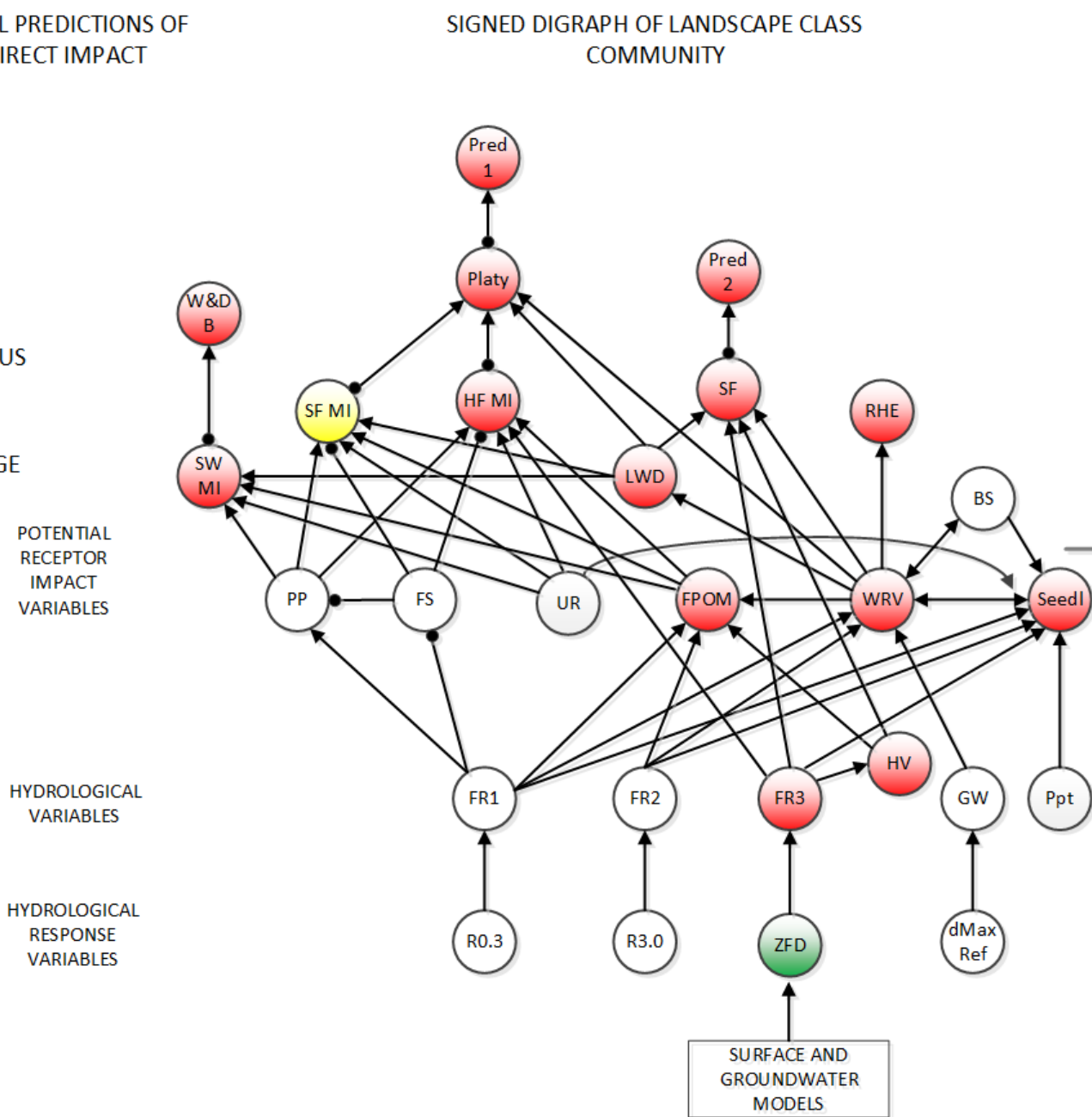
Figure 9 Schematic showing how direct and indirect impacts are qualitatively and quantitatively assessed within the bioregional assessments for an impact scenario of intermediate complexity
